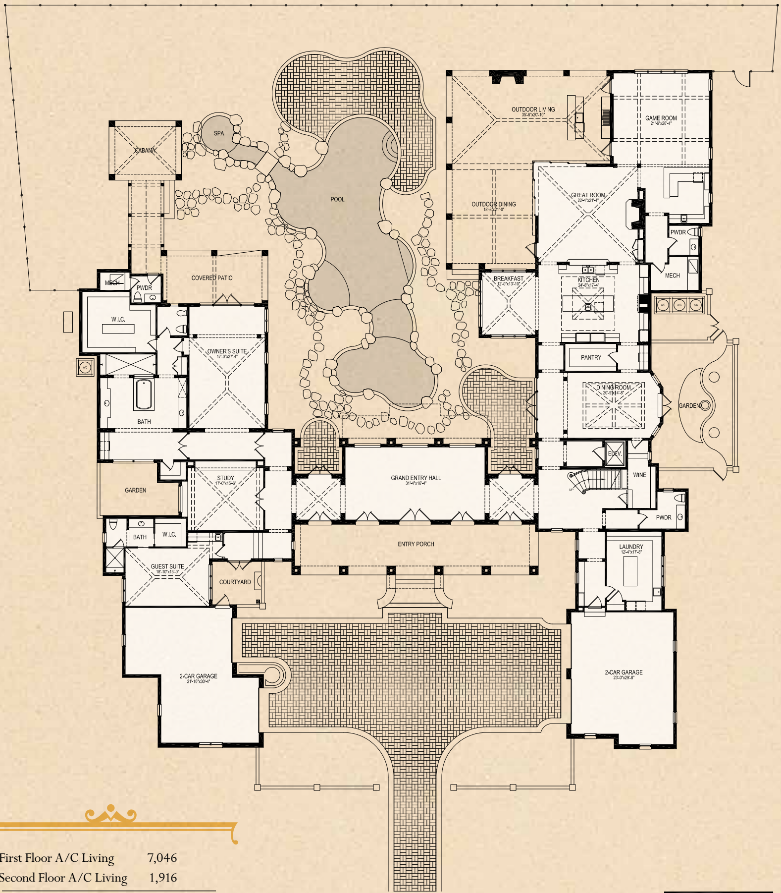
FIRST FLOOR
